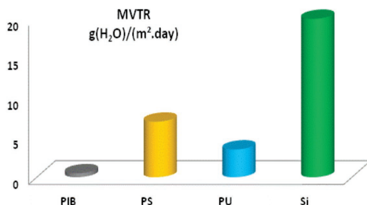
Figure 3: Moisture vapor transmission rates for polyisobutyl (PIB), polysulfide (PS), polyurethane (PU) and silicone (Si) sealants.
