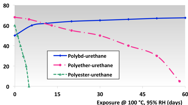
Figure 7: Comparative hydrolytic stability of polyurethanes based on various polyols. 3 A Poly bd-based PU sealant will retain original properties over time.
