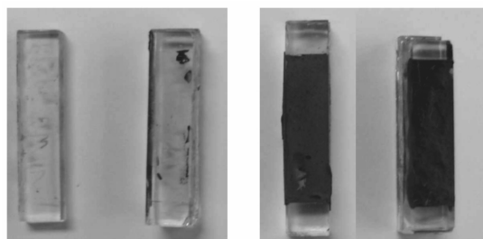
Figure 8: Comparative adhesion to glass after UV exposure of Poly bd-free (left) and Poly bd-based (right) PUs. Only the Poly bd-based PUs maintain good adhesion to glass after UV aging.
