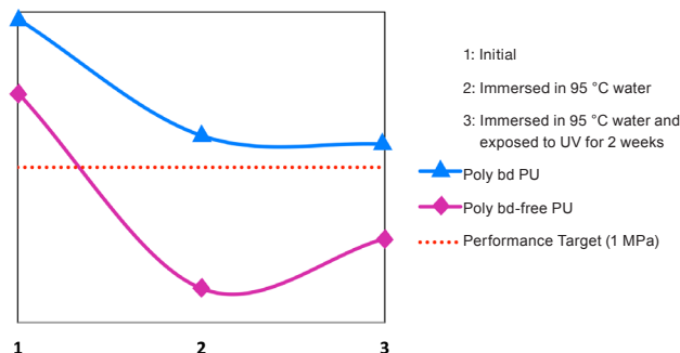
Tensile strength variation during aging
