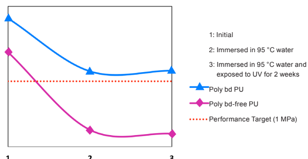
Shear strength variation during aging
