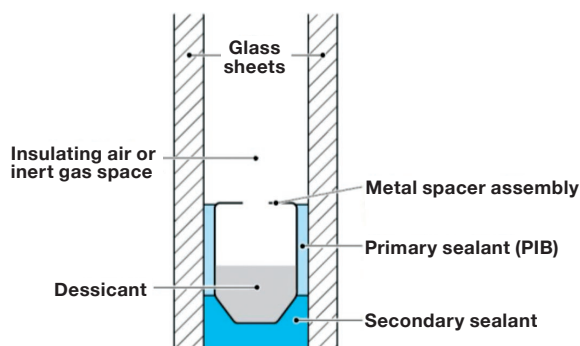
Figure 1: Schema of an insulated glass unit (IGU).
