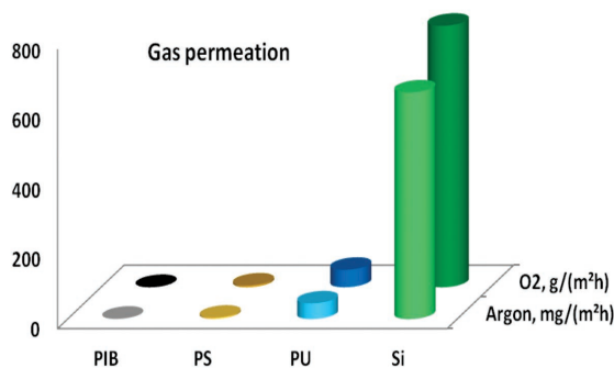
Figure 4: Gas permeation rates for polyisobutyl (PIB), polysulfide (PS), polyurethane (PU) and silicone (Si) sealants.
