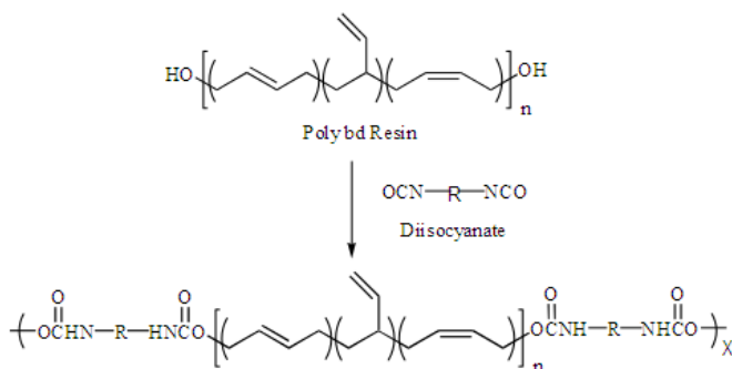
Figure 2: Poly bd-based polyurethane.
